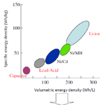
Advantage of Li-ion battery is "Light Weight and Small Volume"
