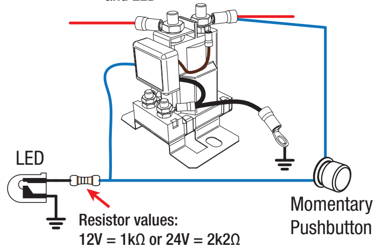
SBI with Push Button and LED
