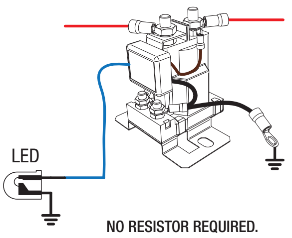
SBI with External LED
