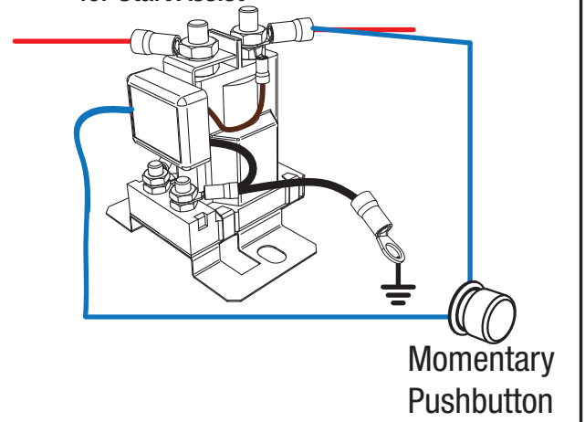
SBI with Push Button for Start Assist
